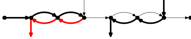
Figure 6. An unbalanced bridge always gives an extra cost of 2.
