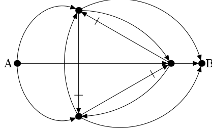
Figure 1. The gadget for equations of the form x + y + z = 0 . There is a Hamiltonian path from A to B only if zero or two of the ticked edges are traversed.
