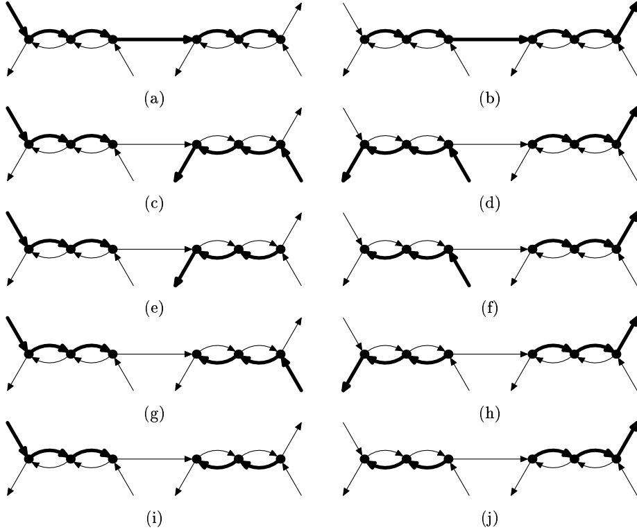
Figure 10. If the negative occurrence in the consistency checker is semitraversed, the checker has to be traversed as shown above.
