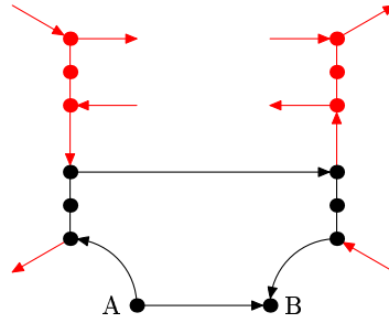
Figure 6. A more detailed view of the gadget for equations of the form x+y=0 . In this figure the ticked edges have been expanded to show the consistency checkers. The black edges correspond to the gadget shown in Fig. 5
