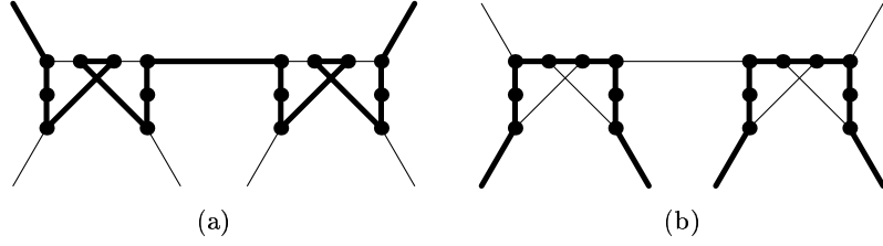
Figure 18. If either the upper two or the lower four connection edges are traversed in the consistency gadget, it is locally optimal to traverse the gadget as shown above.
