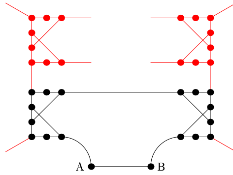
Figure 16. A more detailed view of the gadget for equations of the form x + y + z = 0 . The figure shows how the three variable gadgets meet in the center of the gadget. The black edges above correspond to the ticked edges in Fig. 13 and the three labeled vertices above are the same as the corresponding vertices in Fig. 13.
