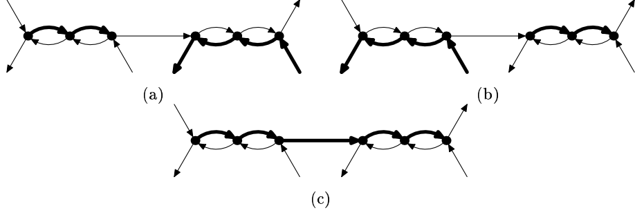
Figure 9. If there are no semitraversed occurrences in the consistency checker but the occurrences are still inconsistent, the checker has to be traversed as shown above.
