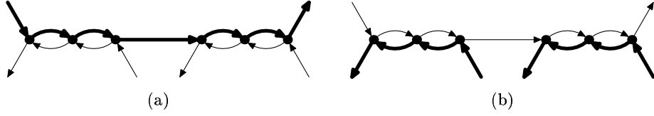
Figure 11. If either the upper two or the lower four connection edges are traversed in the consistency gadget, it is locally optimal to traverse the gadget as shown above.
