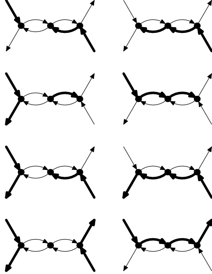
Figure 8. It is possible to change the traversals in the left column into the traversals in the right column without increasing the total number of endpoints in the graph.
