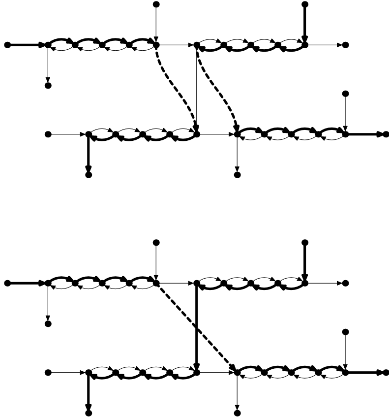
Figure 27. Switching from traversing an edge gadget representing an occurrence of x to traversing another edge gadget representing an occurrence of x gives an extra cost of at least b . The dotted edge above has length 3b ; that gives an extra cost of 2b which is then shared evenly among the two semitraversed edge gadgets.
