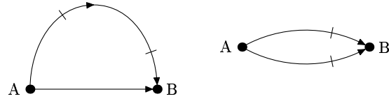
Figure 5. The gadget for equations of the form x+y=0 (left) and x+y=1 (right). There is a Hamiltonian path from A to B only if an even (left) or odd (right) number of the ticked edges is traversed.
