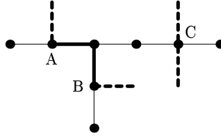
Figure 2. The above figure contains two partial tours—one entering the graph at A and leaving at B , and one both entering and leaving at C . The vertices A and B are endpoints and C is a double endpoint. The dashed parts of the tour denotes parts where the tour traverses edges with weight two.
