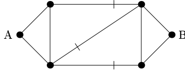
Figure 31. The symmetric gadget for equations of the form x + y + z = 1 . There is a Hamiltonian path from A to B only if zero or two of the ticked edges are traversed.
