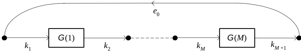
Figure 1: The network \mathcal{N}_r . The edge between \mathcal{G}(i) and \mathcal{G}(i+1) is the output edge of \mathcal{G}(i) and the input edge of \mathcal{G}(i+1) .
