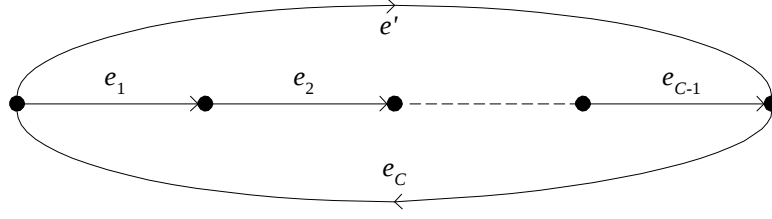
Figure 3: The network \mathcal{B}
