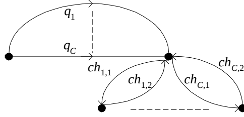
Figure 4: Subnetwork \mathcal{D}
