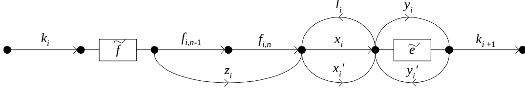
Figure 2: The gadget \mathcal{G}(i)
