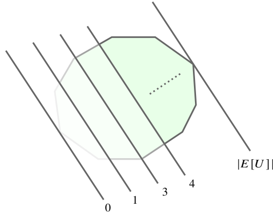
Fig. 1.5 The faces \sum_{e \in E[U]} x_e = \delta for \delta \in [E[U]] of the \text{TS}(G, l) polytope refuted sequentially in the SP refutation.
